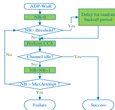
Fig. 3. The working procedure of the ADP-WuR protocol.
