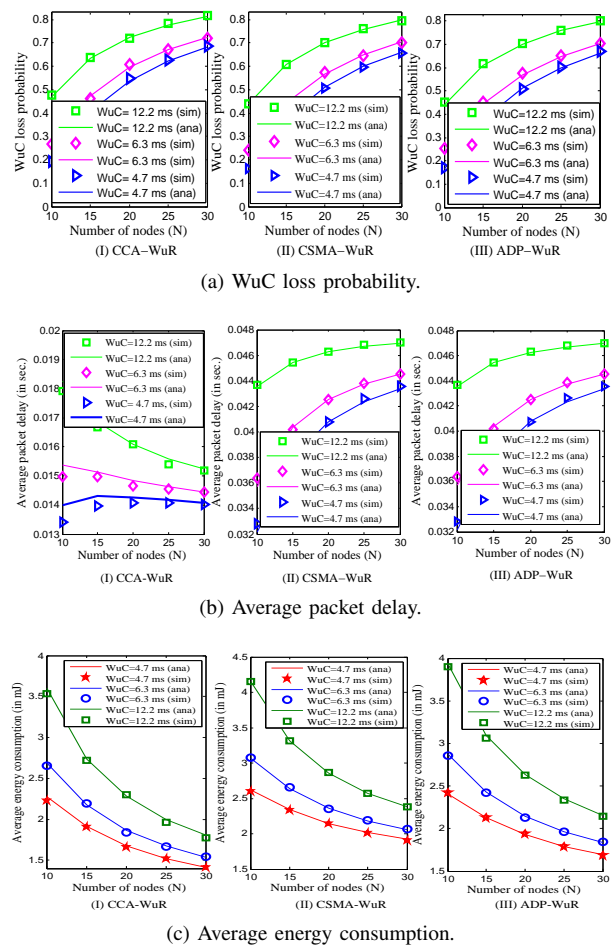
Fig. 10. Effects of data rate and address length for WuC transmissions.
