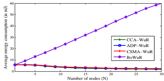
Fig. 12. Average energy consumption comparison of BoWuR, CCA-WuR, CSMA-WuR, and ADP-WuR when the WuC duration is 12.2 ms.
